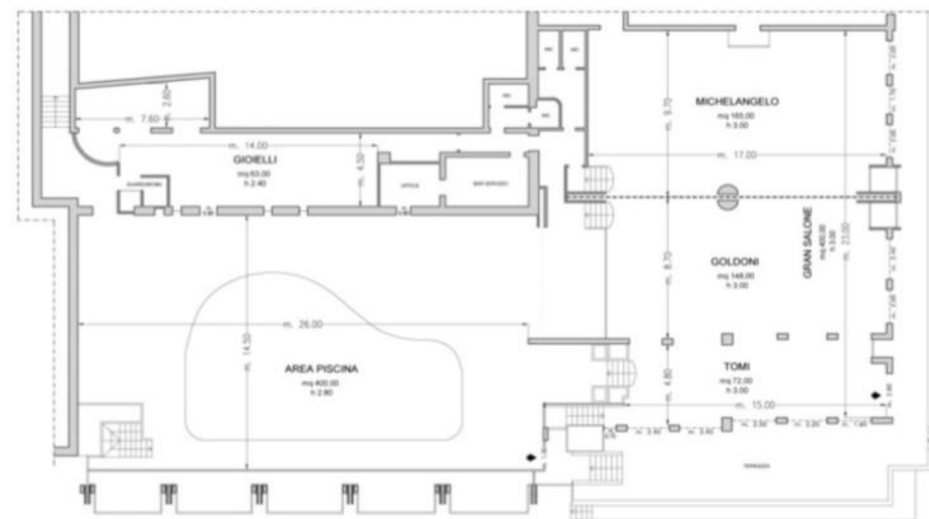
Piano -1 / Basement
